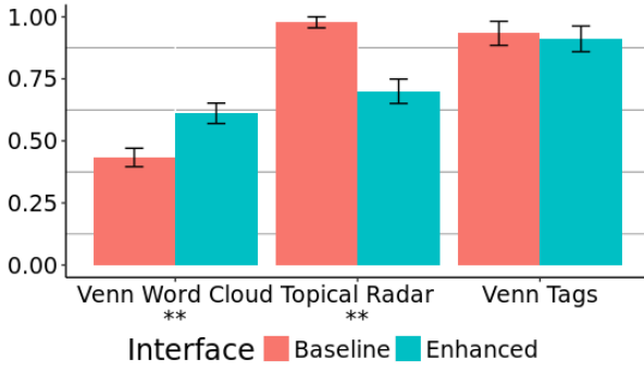
Figure 2: The correct rate of the recommendation-sorting tasks. Statistical significance level: (**) p < 0.01 ; (*) p < 0.05
