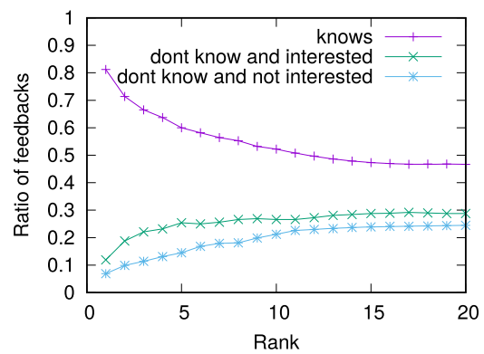
Fig. 4. The distribution of collected feedback types by rank: number of persons whom the user was previously familiar with ('knows'), or otherwise, interested – or not interested – in meeting with.
