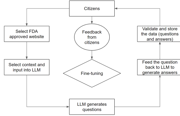
Fig. 1. The iterative citizen-driven data collection and annotation process for LLM fine-tuning.
